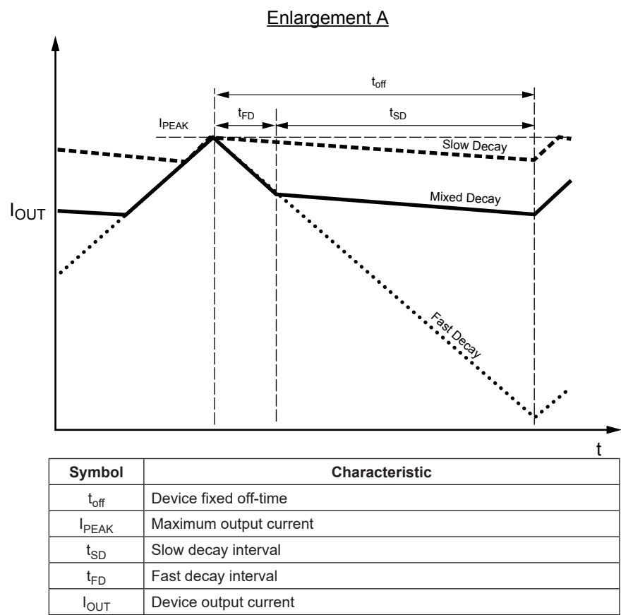
Figure 7: Current Decay Modes Timing Chart
