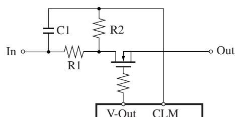
Figure 6. CLM noise filter circuit
