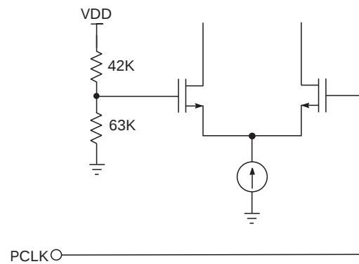
Figure 2-5: PCLK Input
