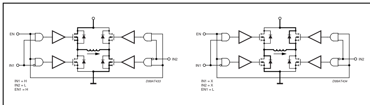
Figure 5c. Enable chopping
