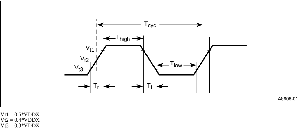
Figure 61. SRAM SCLK Signal AC Parameter Measurements
