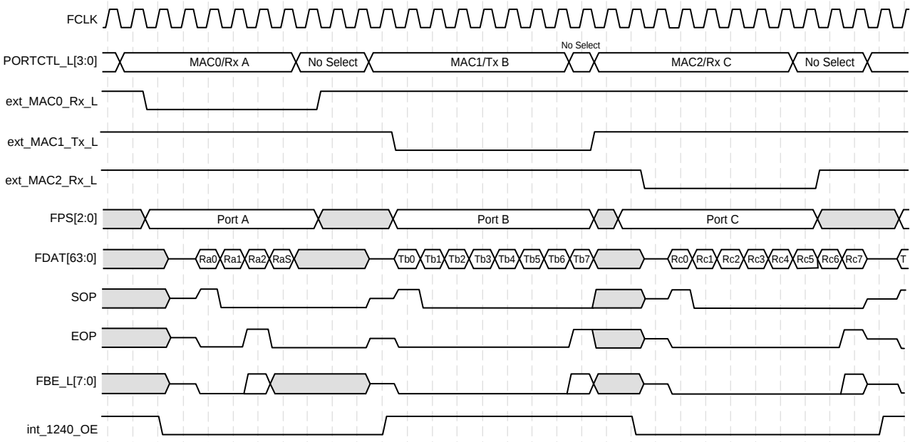
Figure 28. 64-Bit Bidirectional IX Bus Timing - Consecutive Receive and Transmit, EOP on 1st through 3rd Data Return with Status (3rd Data Return Shown)
