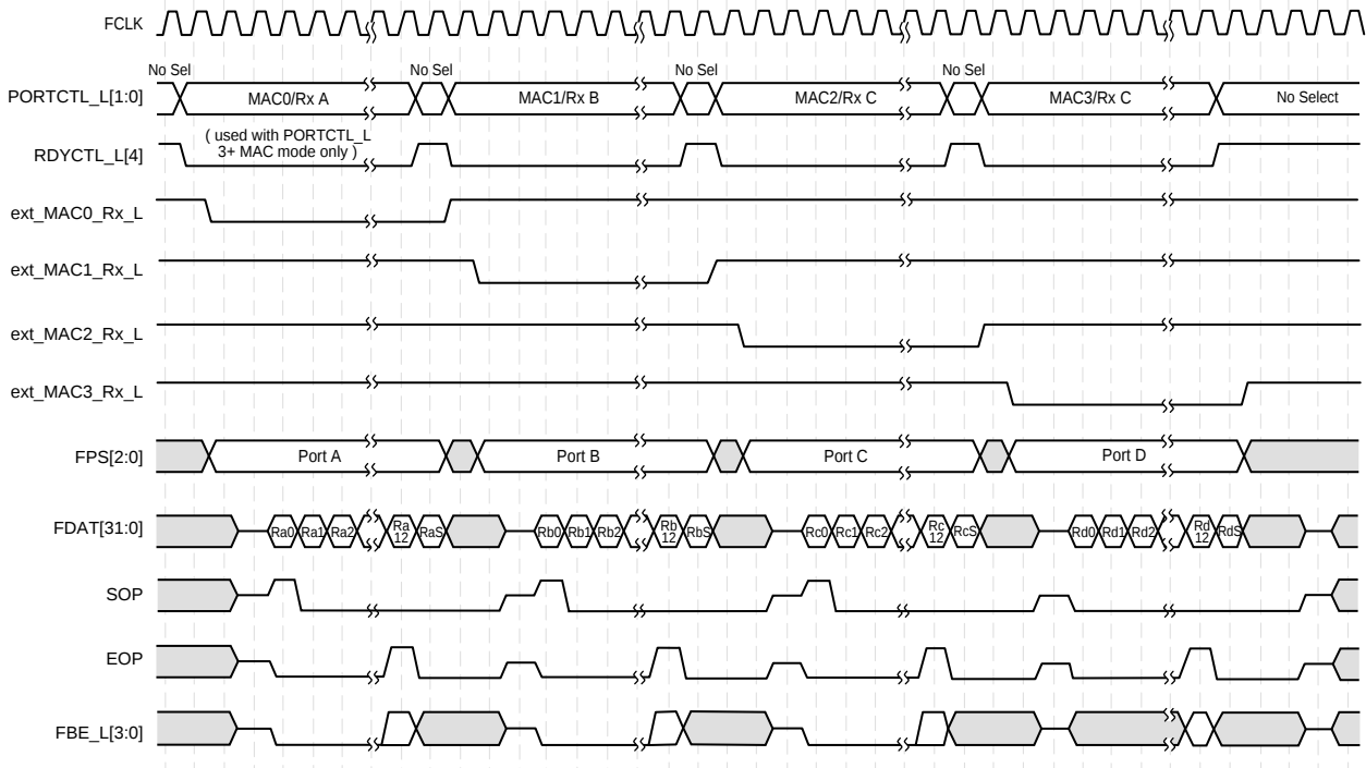
Figure 42. 32-Bit Unidirectional IX Bus Timing - Consecutive Receives, EOP on 1st Through 13th Data Return with Status (13th Data Return Shown)
