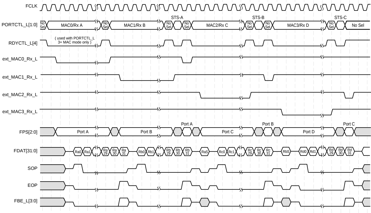
Figure 44. 32-Bit Unidirectional IX Bus Timing - Consecutive Receives, Two Element Transfers with 32-Bit Status
