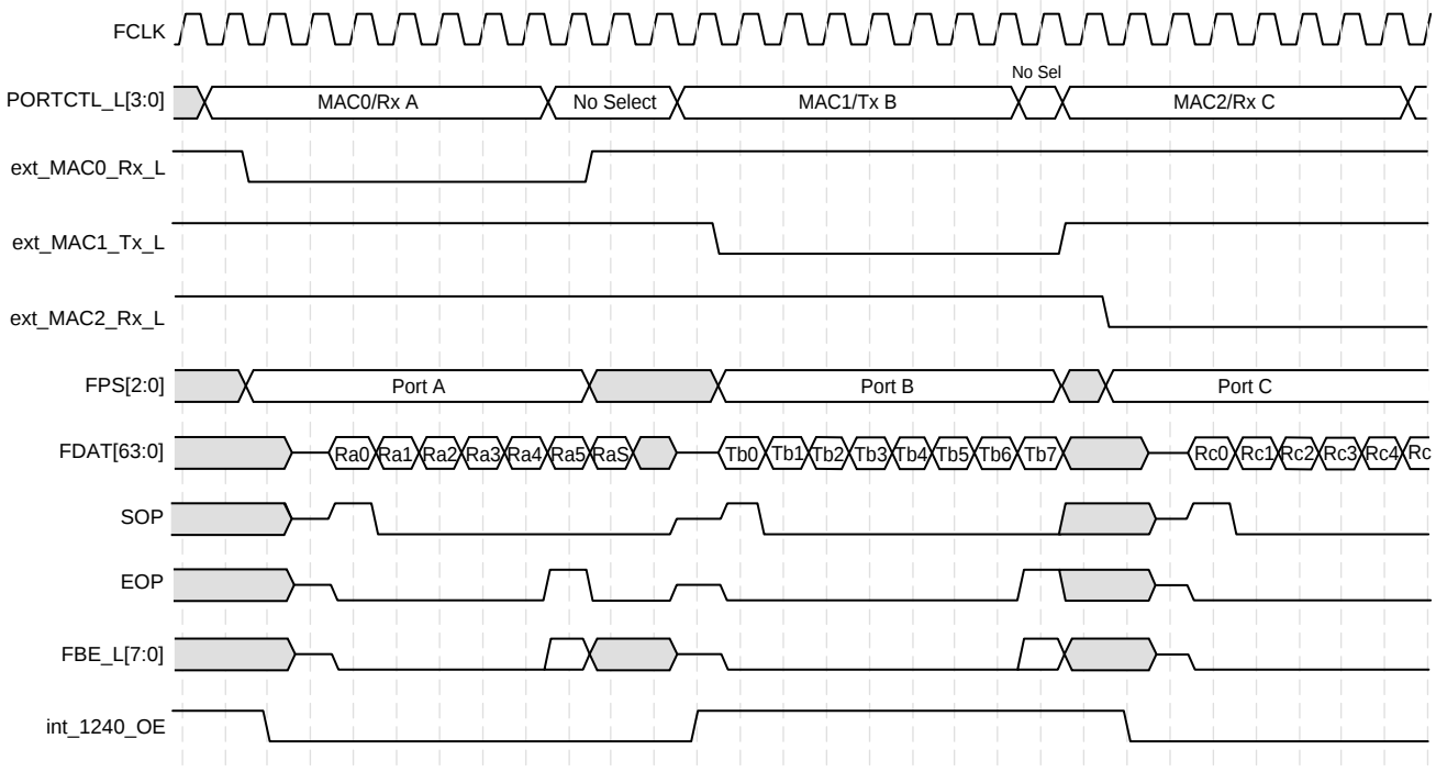
Figure 25. 64-Bit Bidirectional IX Bus Timing - Consecutive Receive and Transmit, EOP on 6th Data Return with Status
