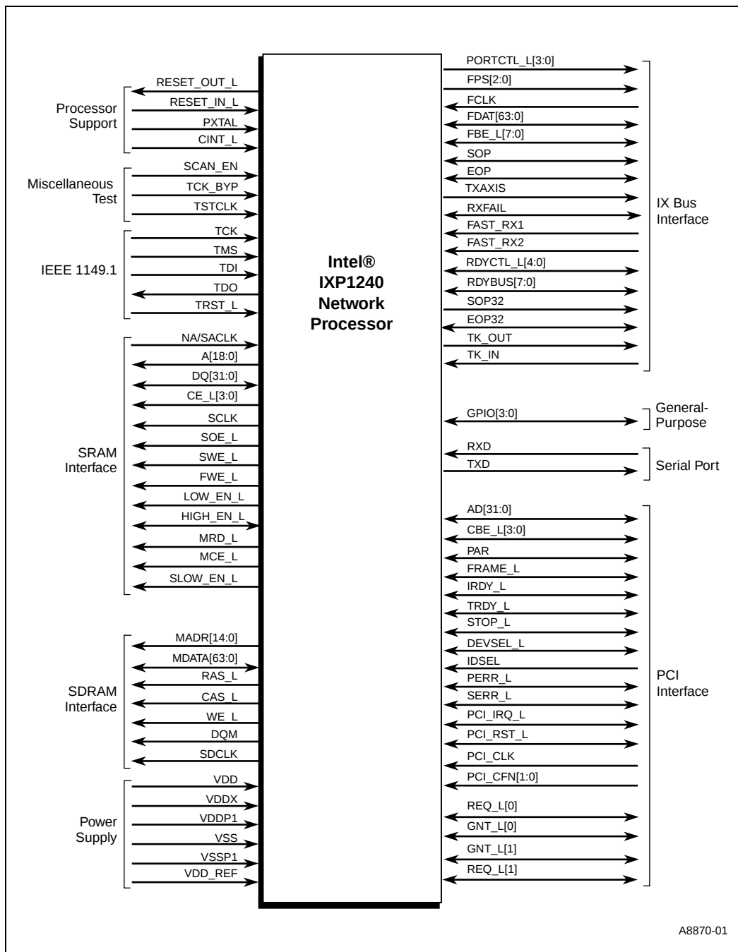
Figure 6. Pinout Diagram
