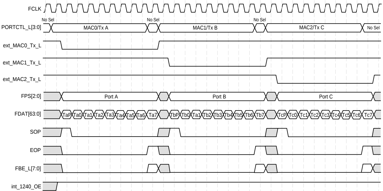
Figure 37. 64-Bit Bidirectional IX Bus Timing - Consecutive Transmits with Prepend, EOP
