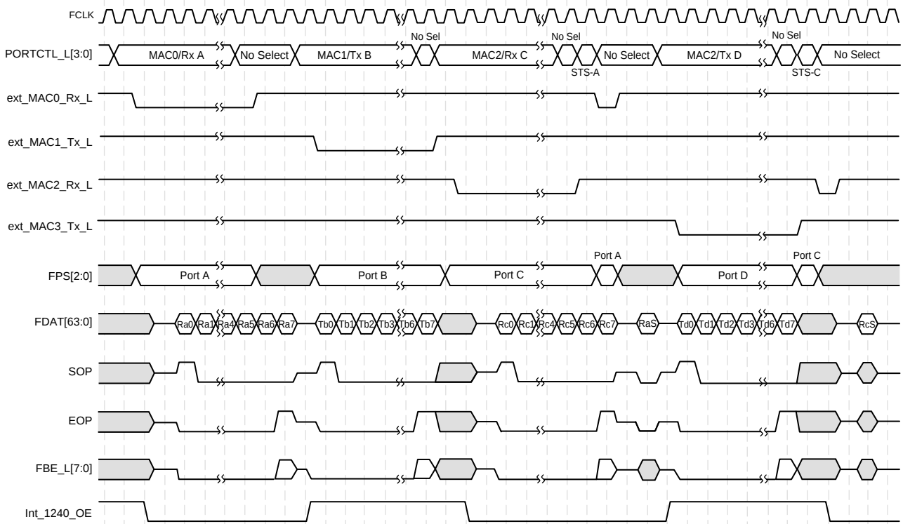
Figure 23. 64-Bit Bidirectional IX Bus Timing - Consecutive Receive and Transmit, EOP on 8th Data Return with Status
