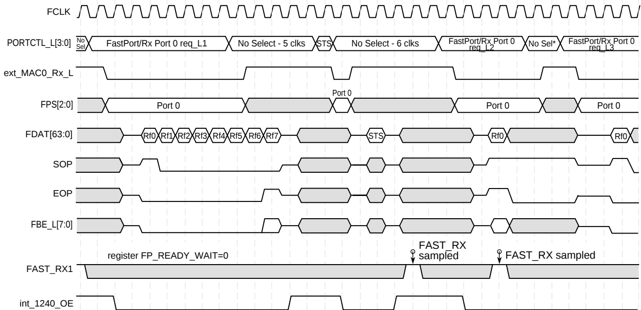
Figure 49. 64-Bit Bidirectional IX Bus Timing - Consecutive FastPort Receives, Same Port, EOP, with Status, FP_READY_WAIT=0
