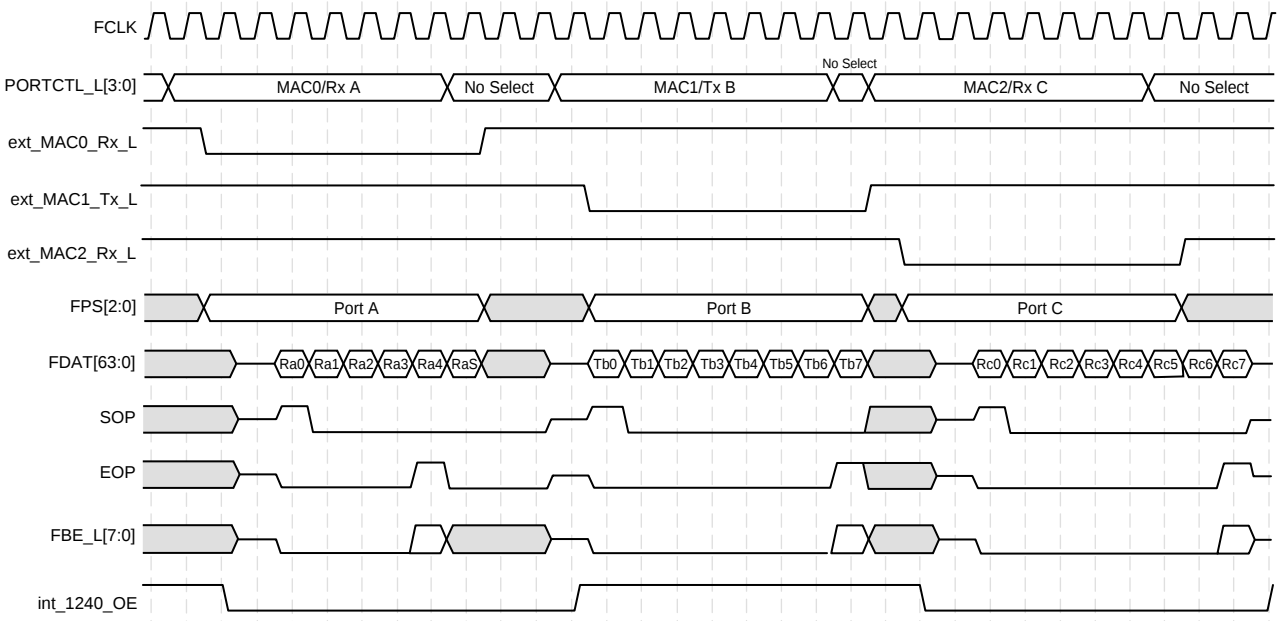
Figure 26. 64-Bit Bidirectional IX Bus Timing - Consecutive Receive and Transmit, EOP on 5th Data Return with Status
