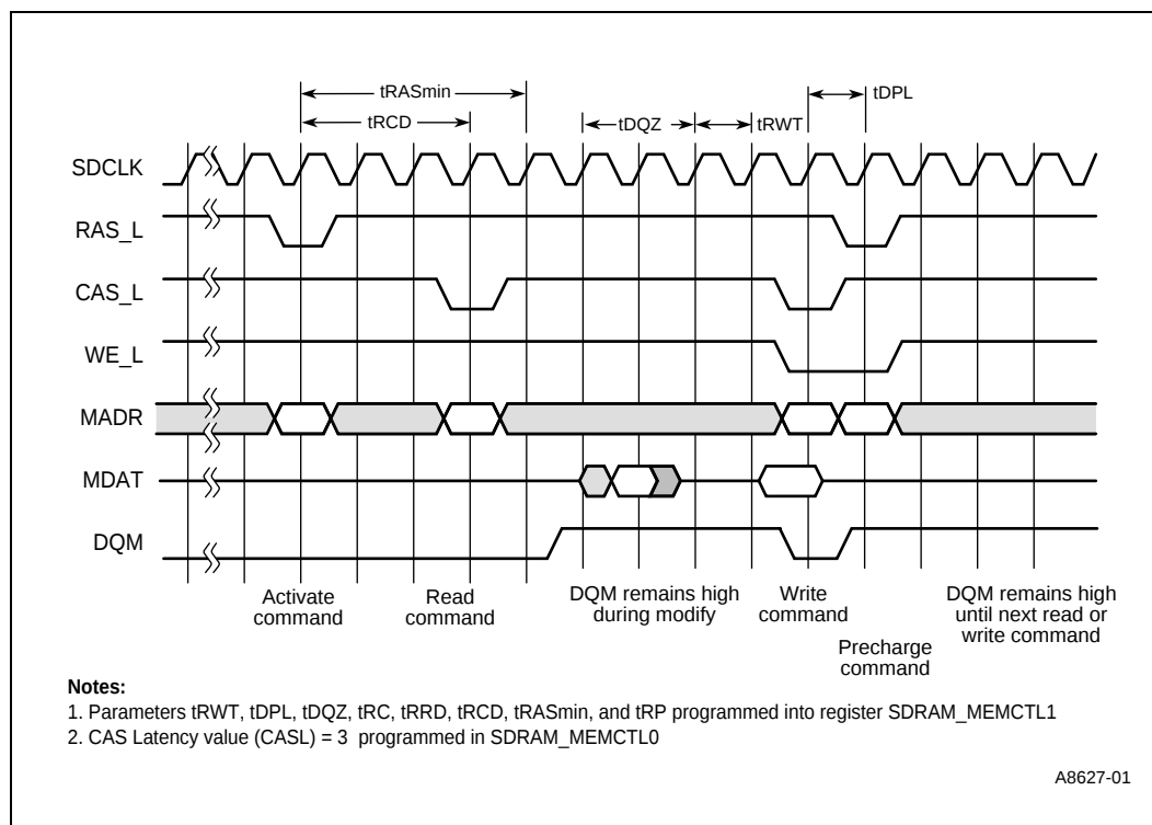
Figure 80. SDRAM Read-Modify-Write Cycle
