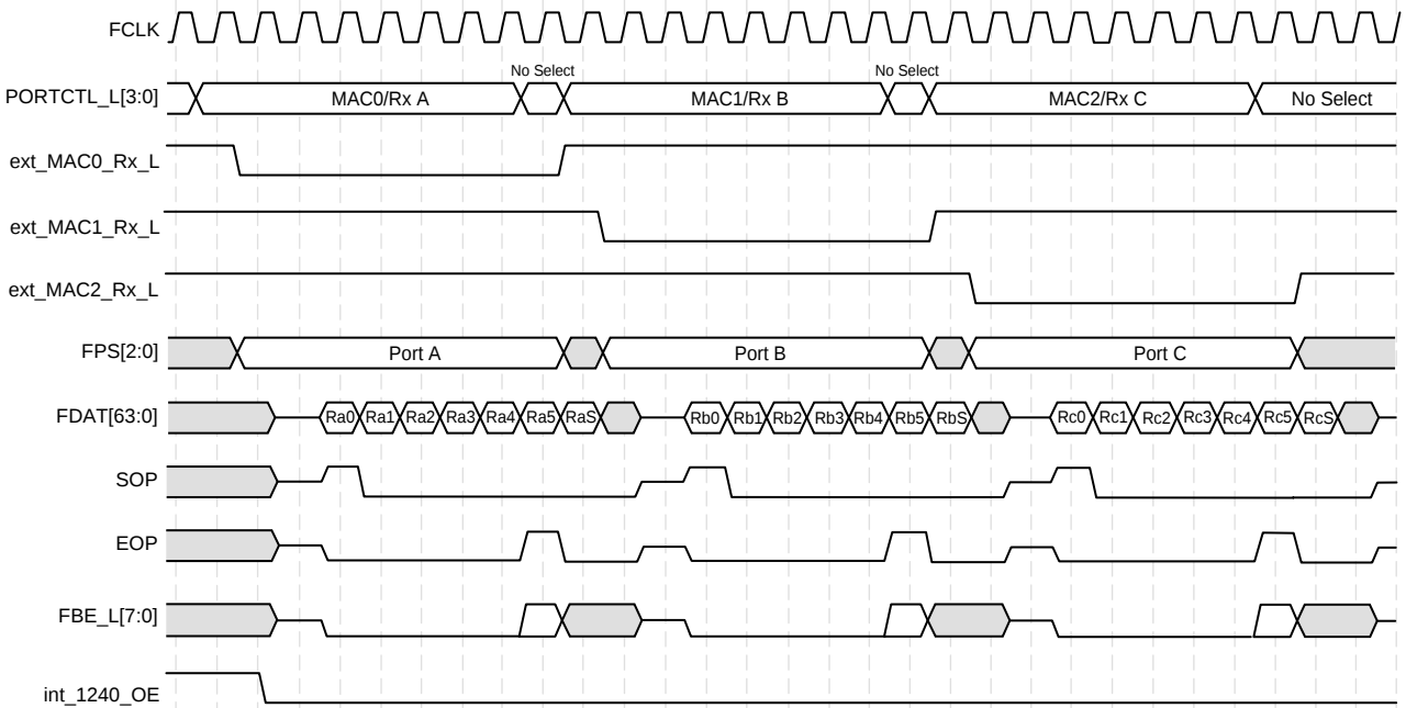
Figure 33. 64-Bit Bidirectional IX Bus Timing - Consecutive Receives, EOP on 6th Data Return with Status
