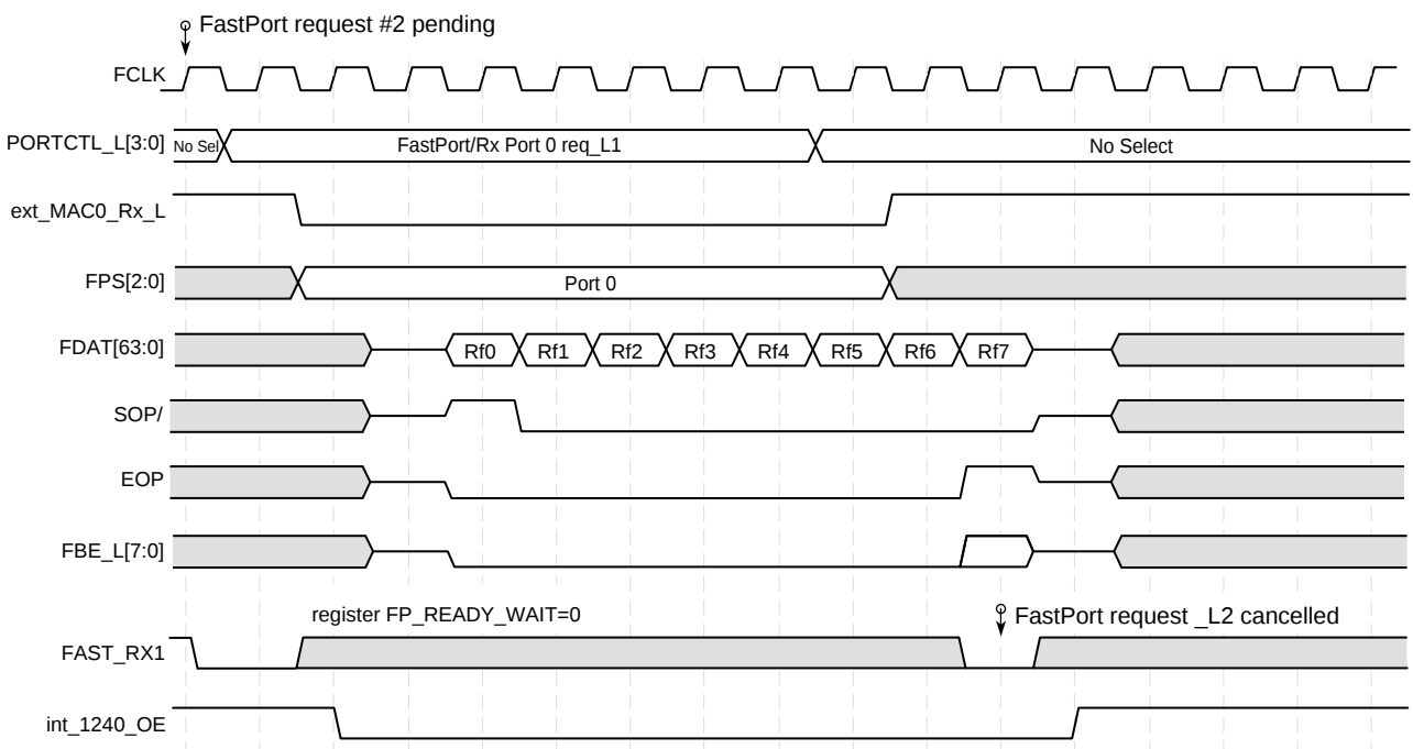
Figure 51. 64-Bit Bidirectional IX Bus Timing - Consecutive FastPort Receives, Same Port, EOP, No Status, FP_READY_WAIT=0, Cancelled Request
