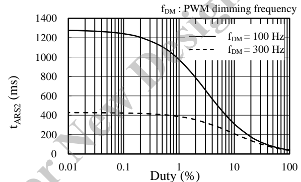
Figure 8-13. PWM Dimming On-duty Versus t_{ARS2}
