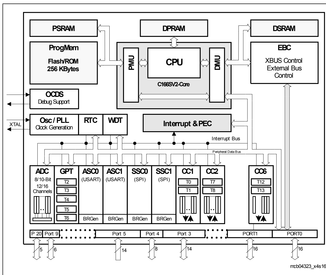
Figure 3 Block Diagram
