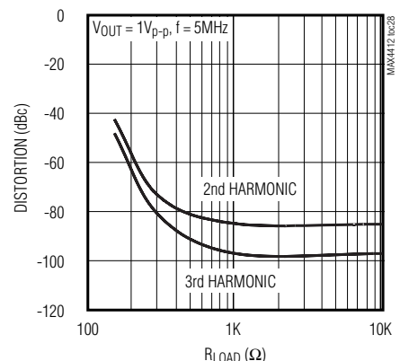
HARMONIC DISTORTION vs. LOAD RESISTANCE
