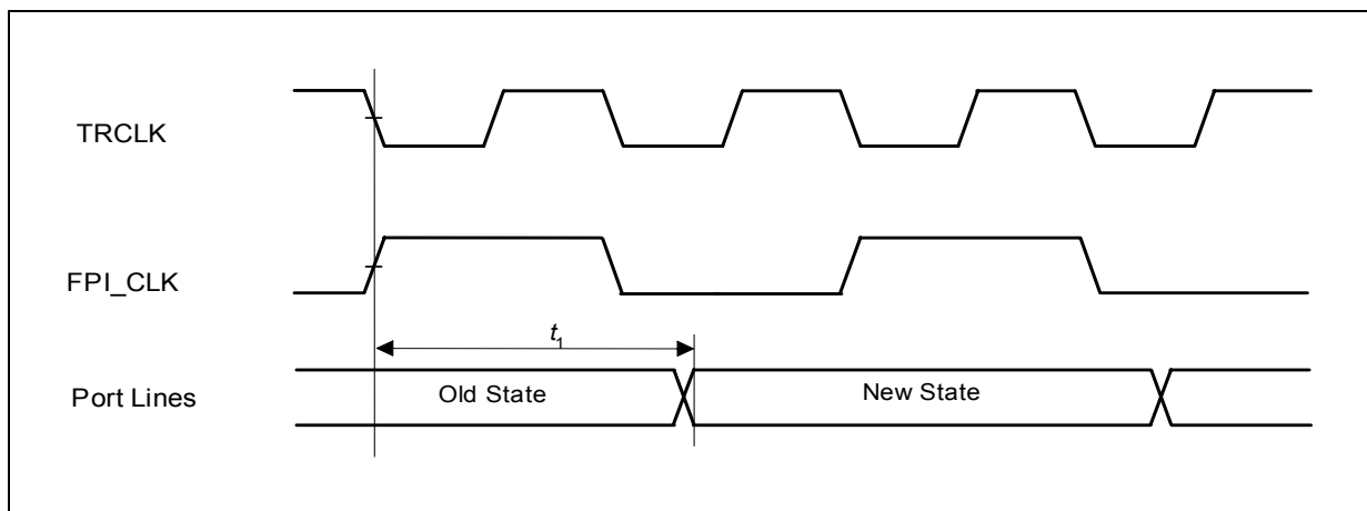
Figure 4-5 Port Timing
