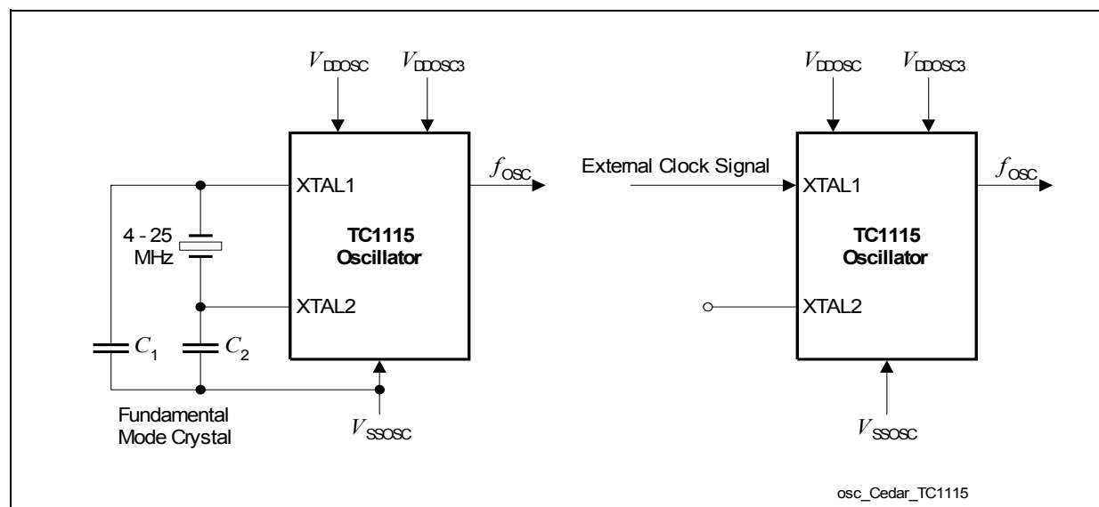
Figure 3-15 Oscillator Circuitries
