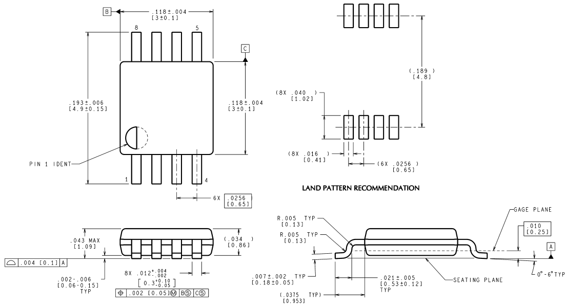
8-Lead (0.118" Wide) Molded Mini Small Outline Package
