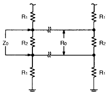
Equivalent Circuit Recommended Termination
