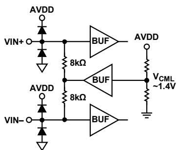
Figure 14. Analog Inputs ( V_{CML} \approx 1.4\text{ V} )
