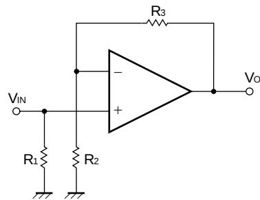
Noninverting Amplifier
