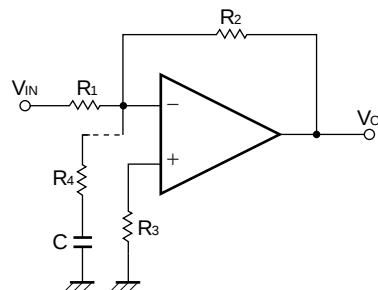
Inverting Amplifier
