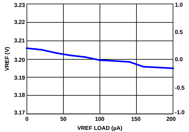
FIGURE 8. VREF LOAD REGULATION
