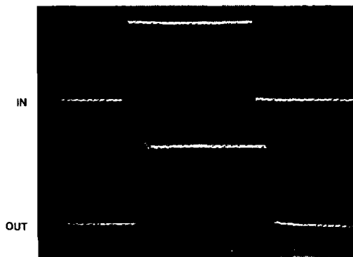
FIGURE 4. VIDEO CABLE DRIVER ( A_{VCL} = 2 )
