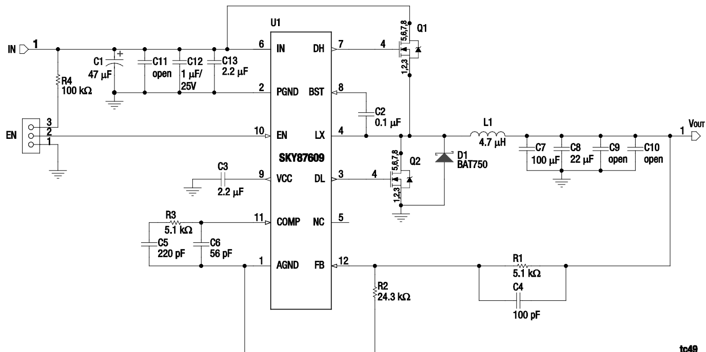
Figure 39: SKY87609 Evaluation Board Schematic
