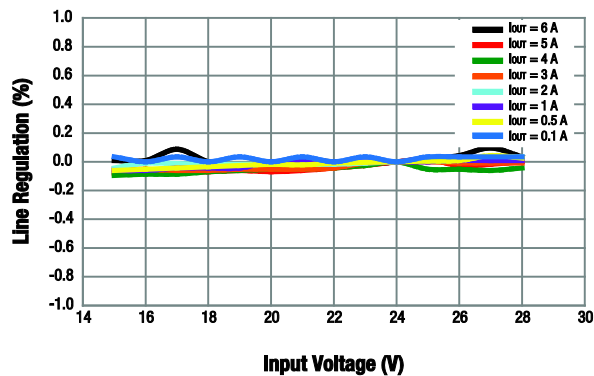
Figure 13. Line Regulation vs Input Voltage ( V_{OUT} = 12\text{ V} )
