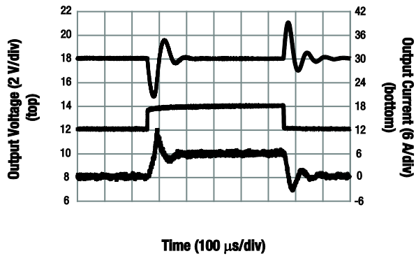
Figure 35. Load Transient ( V_{OUT} = 18 V, V_{IN} = 24 V, I_{OUT} = 0.1 to 6 A)
