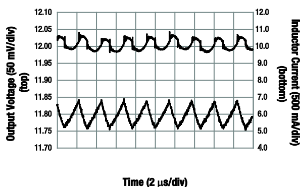
Figure 28. Output Voltage Ripple ( V_{OUT} = 15\text{ V} , V_{IN} = 24\text{ V} , I_{OUT} = 6\text{ A} )
