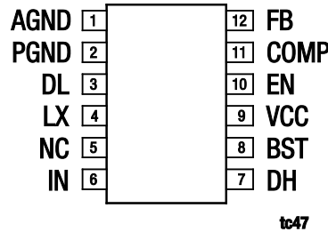
Figure 2. SKY87609 12-Pin TSOPJW (Top View)
