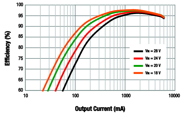
Figure 6. Efficiency vs Output Current ( V_{OUT} = 15\text{ V} )
