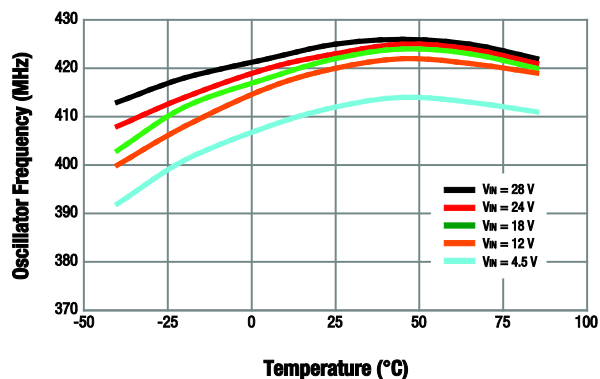
Figure 16. Oscillator Frequency vs Temperature ( I_{OUT} = 100\text{ mA} )
