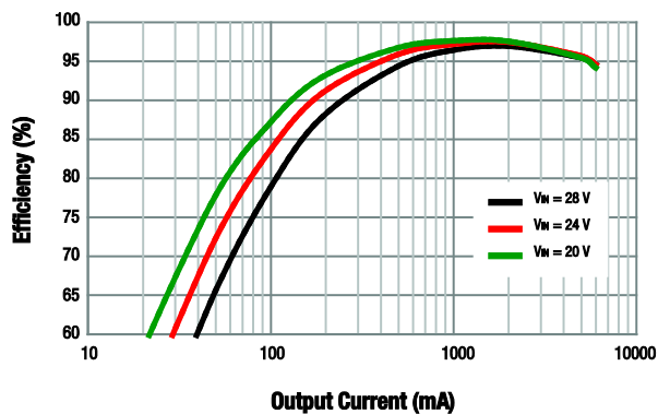
Figure 7. Efficiency vs Output Current ( V_{OUT} = 18\text{ V} )
