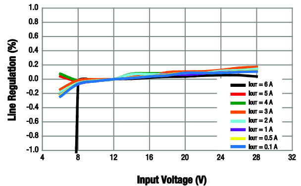
Figure 12. Line Regulation vs Input Voltage ( V_{OUT} = 3.3\text{ V} )
