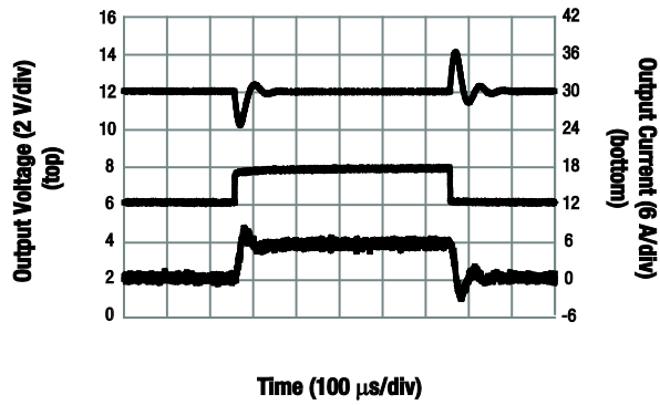
Figure 33. Load Transient ( V_{OUT} = 12 V, V_{IN} = 24 V, I_{OUT} = 0.1 to 6 A)
