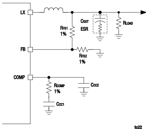
Figure 38. Compensation Components
