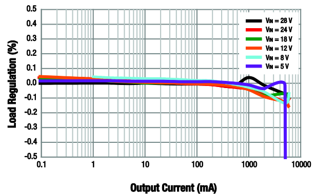
Figure 8. Load Regulation vs Output Current ( V_{OUT} = 3.3\text{ V} )
