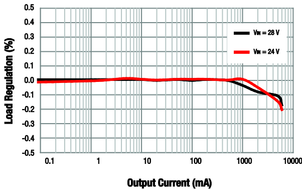
Figure 11. Load Regulation vs Output Current ( V_{OUT} = 18\text{ V} )
