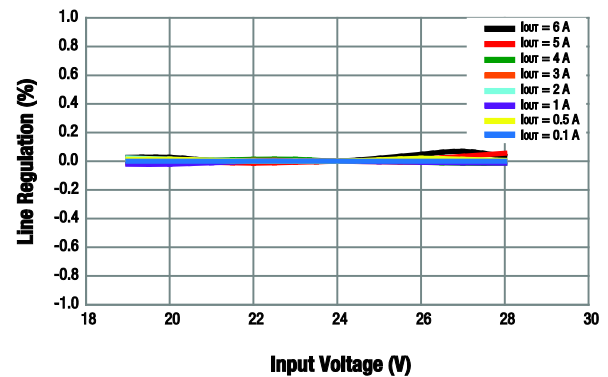
Figure 14. Line Regulation vs Input Voltage ( V_{OUT} = 15\text{ V} )
