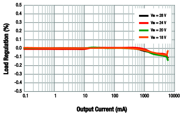
Figure 9. Load Regulation vs Output Current ( V_{OUT} = 12\text{ V} )
