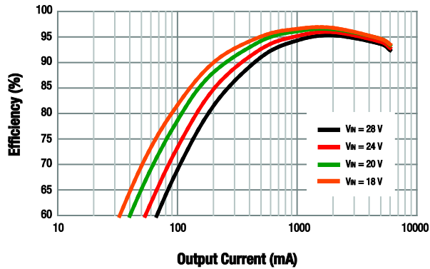
Figure 5. Efficiency vs Output Current ( V_{OUT} = 12\text{ V} )
