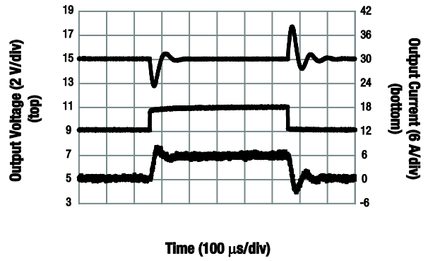
Figure 34. Load Transient ( V_{OUT} = 15 V, V_{IN} = 24 V, I_{OUT} = 0.1 to 6 A)
