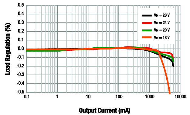
Figure 10. Load Regulation vs Output Current ( V_{OUT} = 15\text{ V} )
