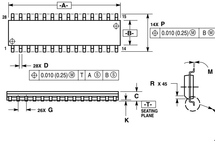
Figure 20-4. 28-Pin SOIC (Case #751F)
