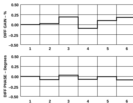
Figure 9. Differential Gain/Differential Phase
