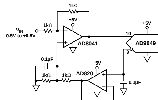
Figure 16. Single Supply, Single Ended, DC Coupled AD9049
