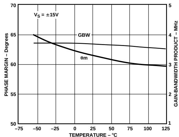
TPC 18. Gain Bandwidth Product and Phase Margin vs. Temperature @ \pm 15\text{V}
