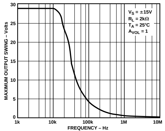
TPC 25. Maximum Output Swing vs. Frequency @ \pm 15 V
