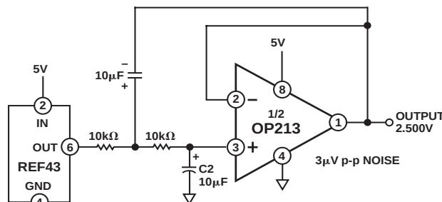
Figure 7. Low Noise Voltage Reference
