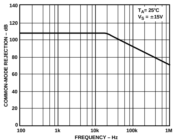
TPC 20. Common-Mode Rejection vs. Frequency @ \pm 15\text{V}
