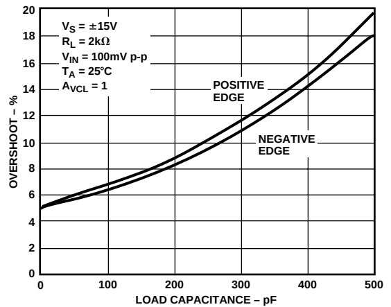
TPC 26. Small Signal Overshoot vs. Load Capacitance @ \pm 15 V
