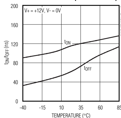
TURN-ON/TURN-OFF TIME vs. TEMPERATURE (SINGLE SUPPLY)
