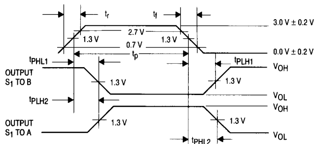
WAVEFORMS
