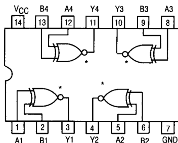
LOGIC DIAGRAM
