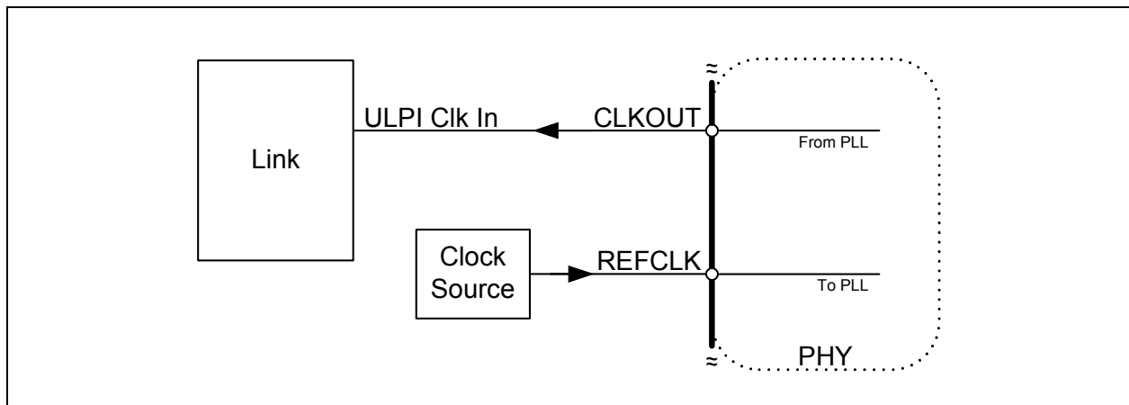
FIGURE 5-4: CONFIGURING THE USB333X FOR ULPI CLOCK OUTPUT MODE
