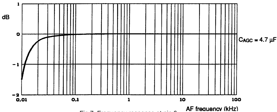
Fig.7 Frequency response at pin 6.
