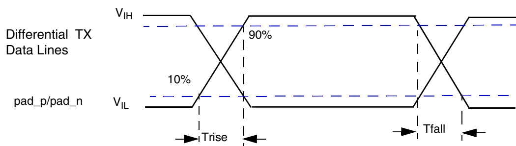
Figure 20. Rise/fall time
