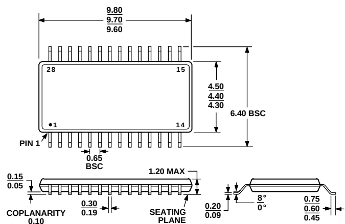
Figure 19. 28-Lead Thin Shrink Small Outline Package [TSSOP] (RU-28) Dimensions shown in millimeters
