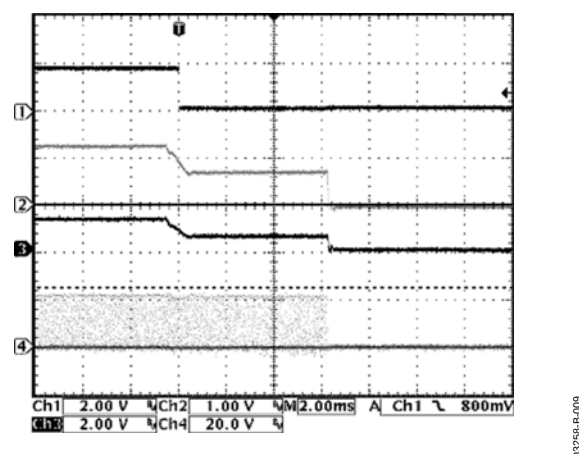
Figure 9. Overcurrent Latch-Off Waveforms, Circuit of Figure 11. Channel 1—PWRGD, Channel 2— V_{OUT} , Channel 3—CSCOMP Pin of ADP3168, Channel 4—High-Side MOSFET V_{GS}
