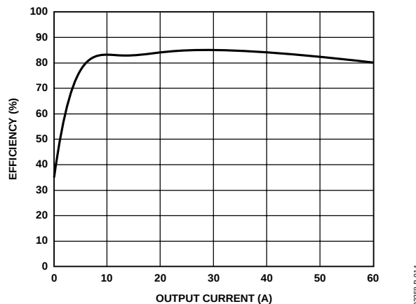
Figure 14. Efficiency of the Circuit of Figure 11 vs. Output Current
