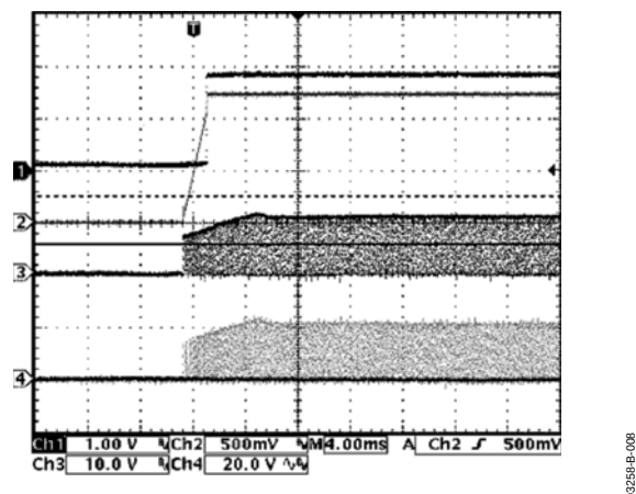
Figure 8. Start-Up Waveforms, Circuit of Figure 12. Channel 1—PWRGD, Channel 2— V_{OUT} , Channel 3—High-Side MOSFET V_{GS} , Channel 4—Low-Side MOSFET V_{GS}
