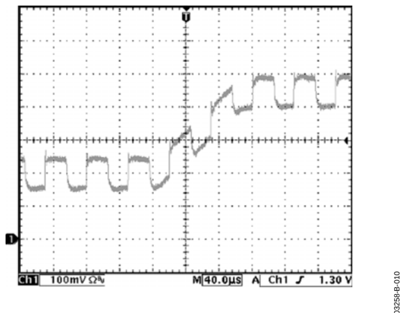
Figure 10. VID On-the-Fly Waveforms, Circuit of Figure 12. VID Change = 5 mV, 5 \mu s per Step, 50 Steps, I_{OUT} Change = 5 A to 65 A
