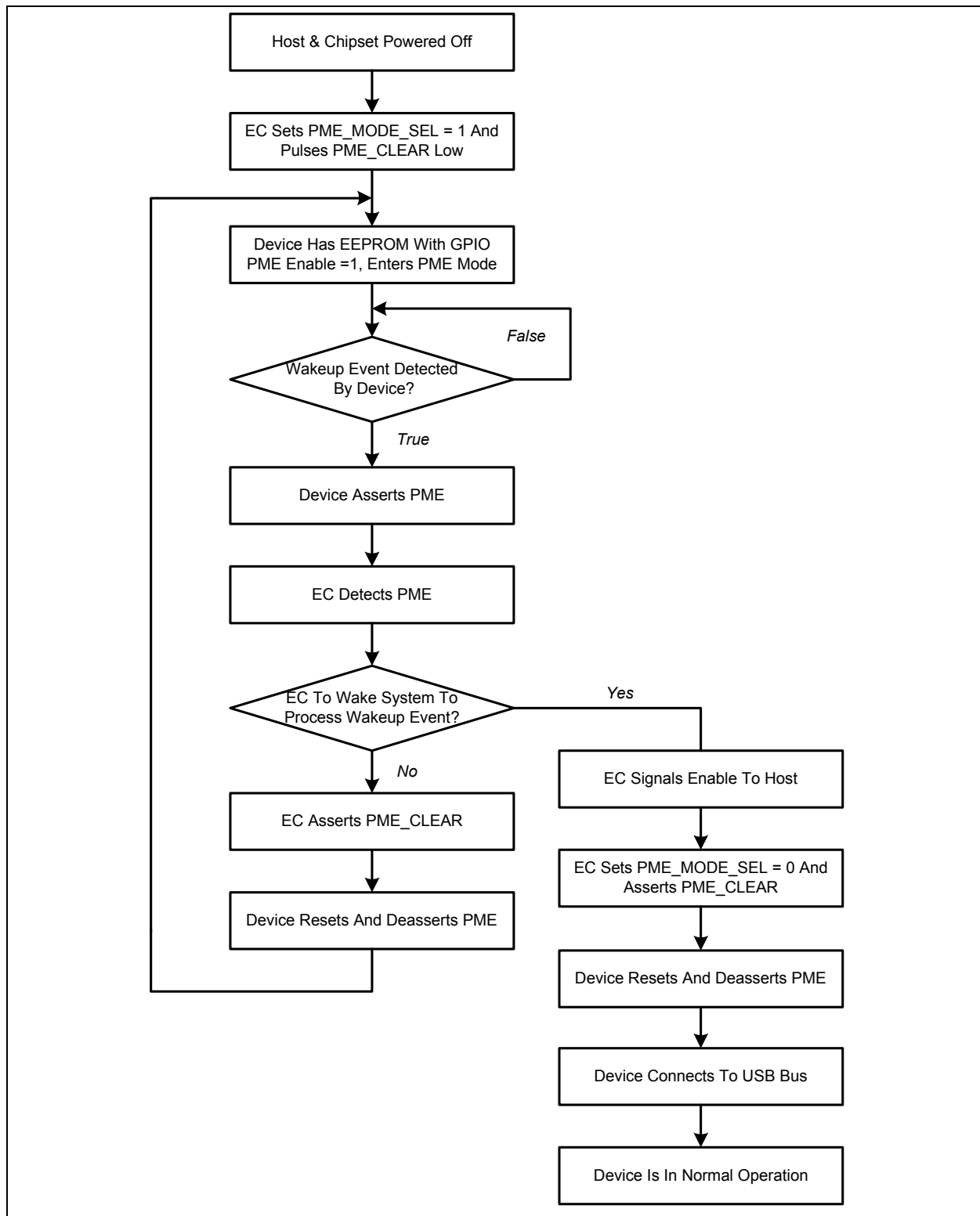
FIGURE 5-2: PME OPERATION
