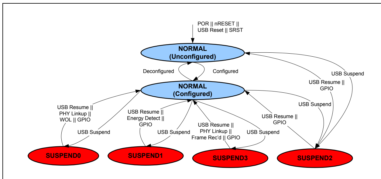
FIGURE 4-29: POWER STATES
