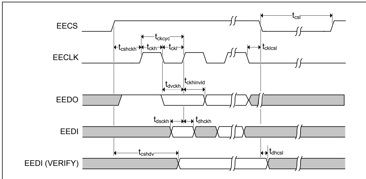
FIGURE 7-5: EEPROM TIMING
