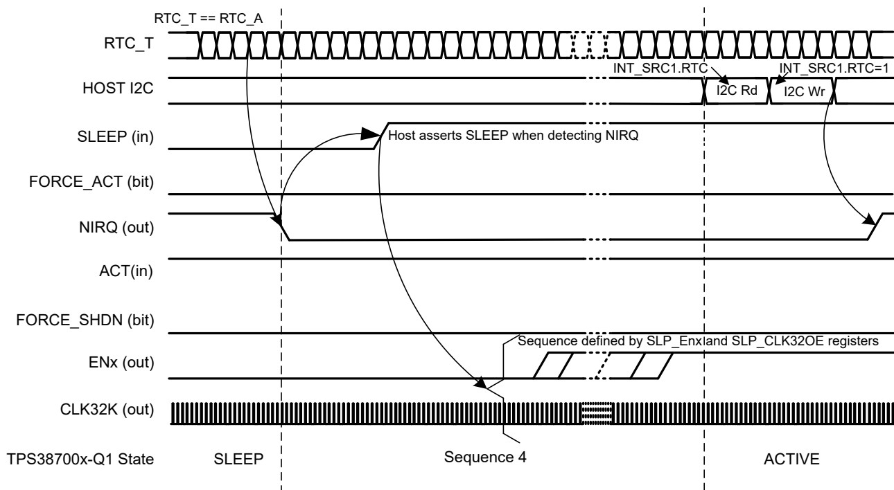
Figure 8-10. Sleep Exit RTC Triggered - \overline{\text{SLEEP}} Sequencing
