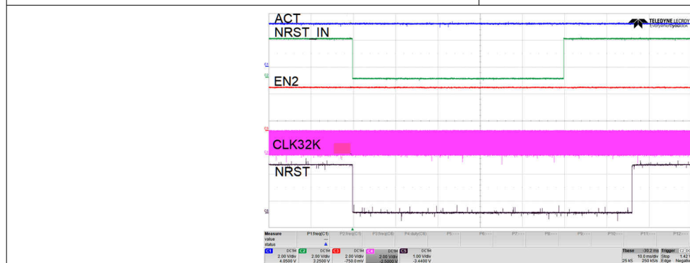
Figure 9-6. RESET Triggered by NRST_IN
