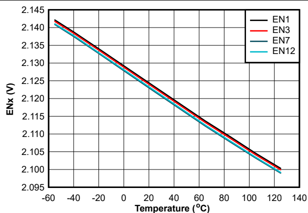
Figure 7-8. ENx Logic High Output Voltage vs. Temperature
