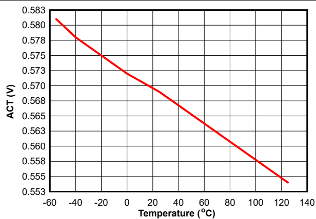
Figure 7-2. ACT Logic Low Threshold Voltage vs. Temperature
