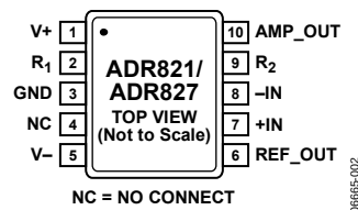
Figure 2. Pin Configuration
