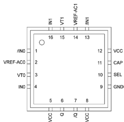
16-Pin QFN
