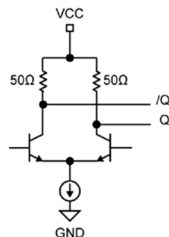
Figure 2b. Simplified Differential Input Stage
