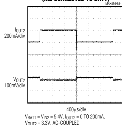
REG2 LOAD-TRANSIENT RESPONSE (IN2 CONNECTED TO BATT)
