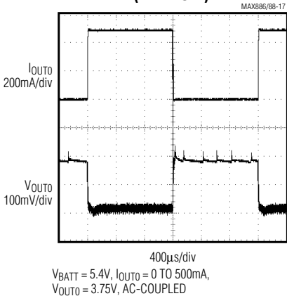
REG0 LOAD-TRANSIENT RESPONSE (PFM MODE)
