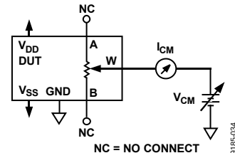
Figure 33. Common-Mode Leakage Current
