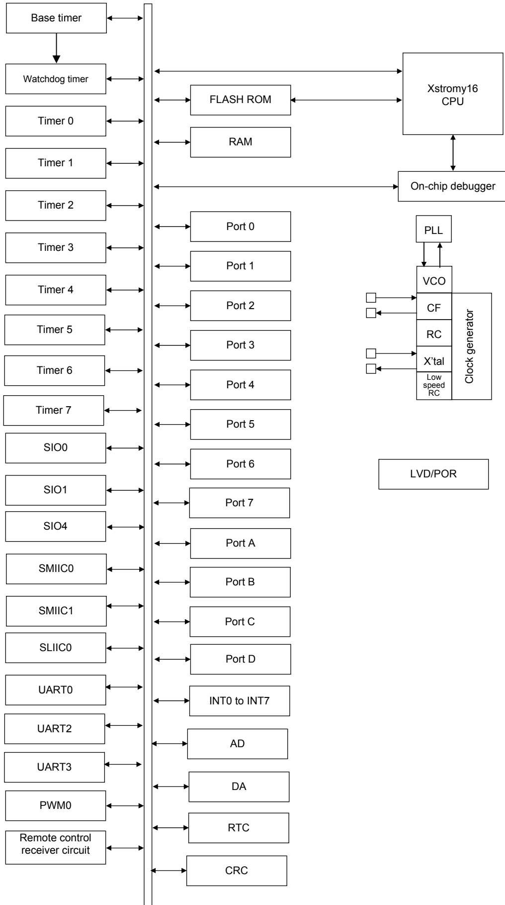
System Block Diagram
