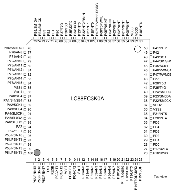
Pin Assignment (Top view)
