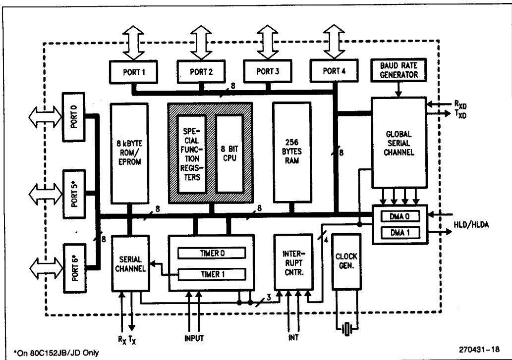
Figure 2. Block Diagram
