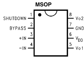
Top View Order Number LM4902MM See NS Package Number MUA08A
