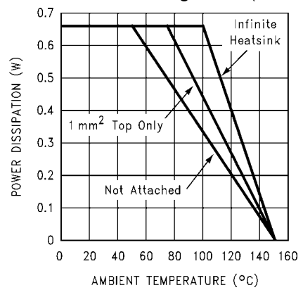
LM4902LD Power Derating Curve (Note 12)
