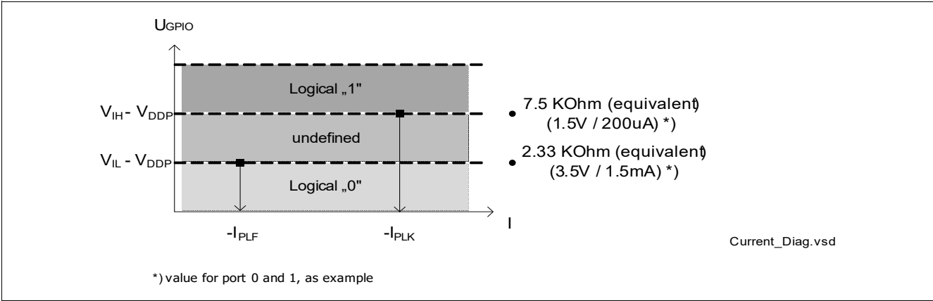
Figure 37 Pull-Up/Down Device
