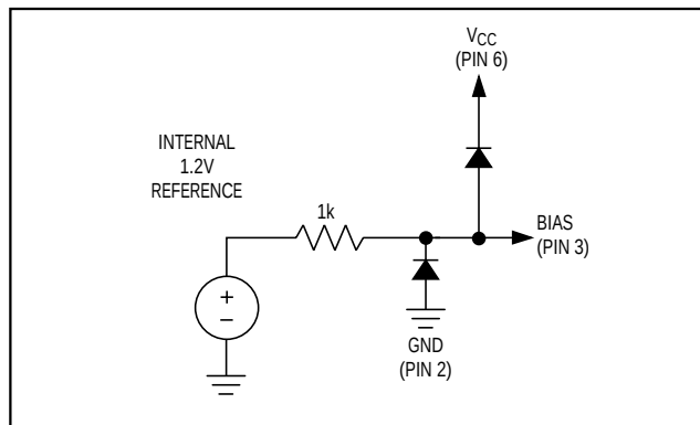
Figure 3. BIAS Structure (MAX2473 only)
