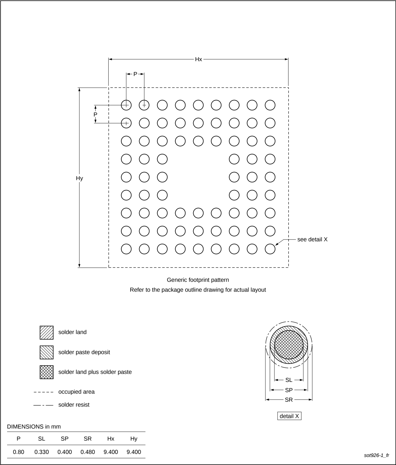
Footprint information for reflow soldering of TFBGA100 package SOT926-1
