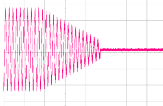
Current Waveform of Soft Off
