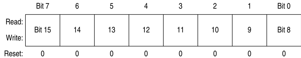
Figure 10-11 Timer Channel Value Register High (TPM1CnVH)
