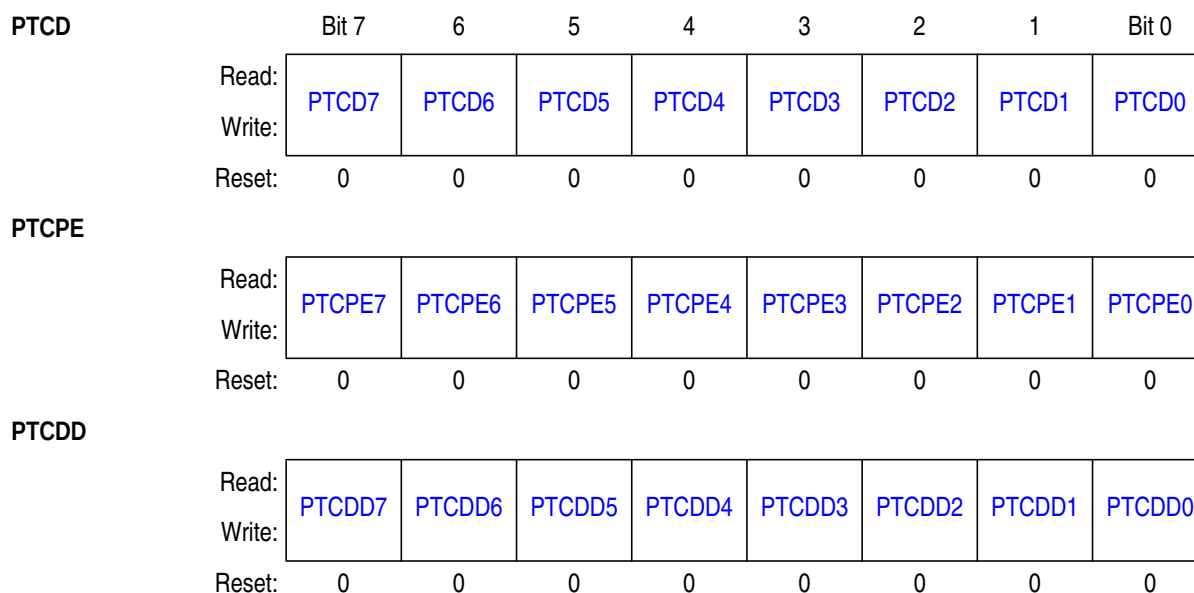
Figure 8-8 Port C Registers
