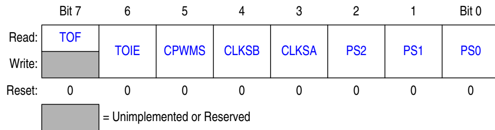
Figure 10-5 Timer Status and Control Register (TPM1SC)
