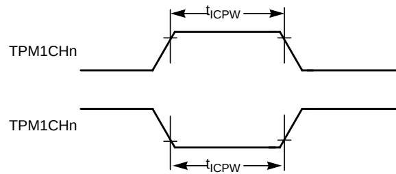
Figure A-10 Timer Input Capture Pulse
