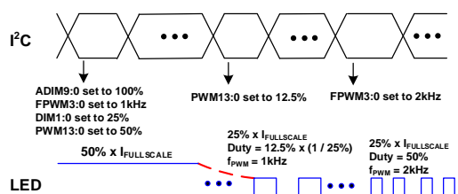
Figure 14: Mixed Dimming from the I 2 C Interface
