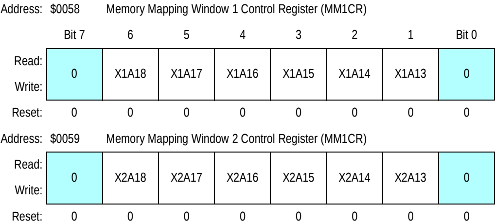
Figure 11-4. Memory Mapping Window Control Registers (MM1CR and MM2CR)
