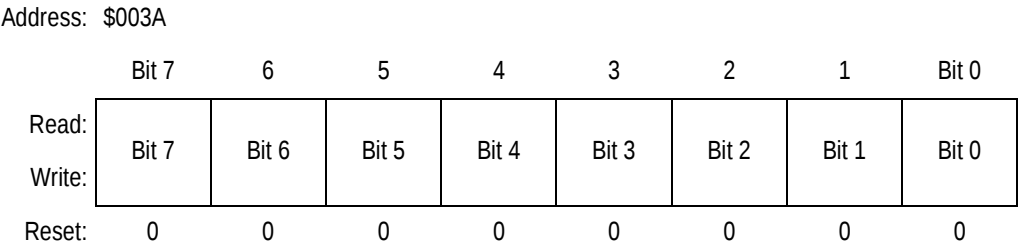
Figure 5-3. Arm/Reset COP Timer Circuitry Register (COPRST)
