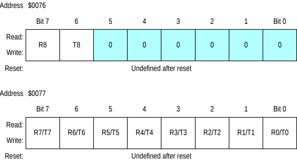
Figure 7-11. SCI Data Register (SCDR)
