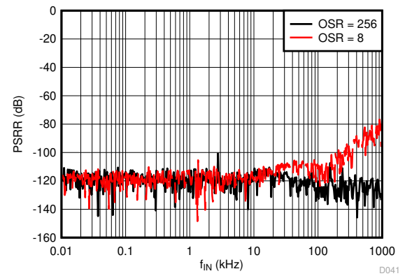
Figure 6-37. Power-Supply Rejection Ratio vs Ripple Frequency
