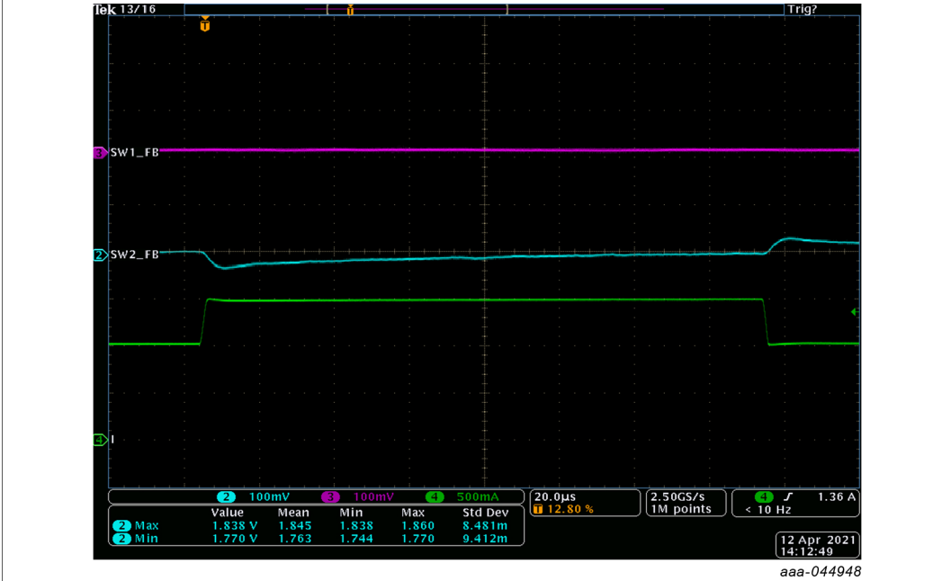
Figure 22. SW2 Load Transient Response
