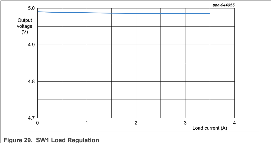
Figure 29. SW1 Load Regulation
