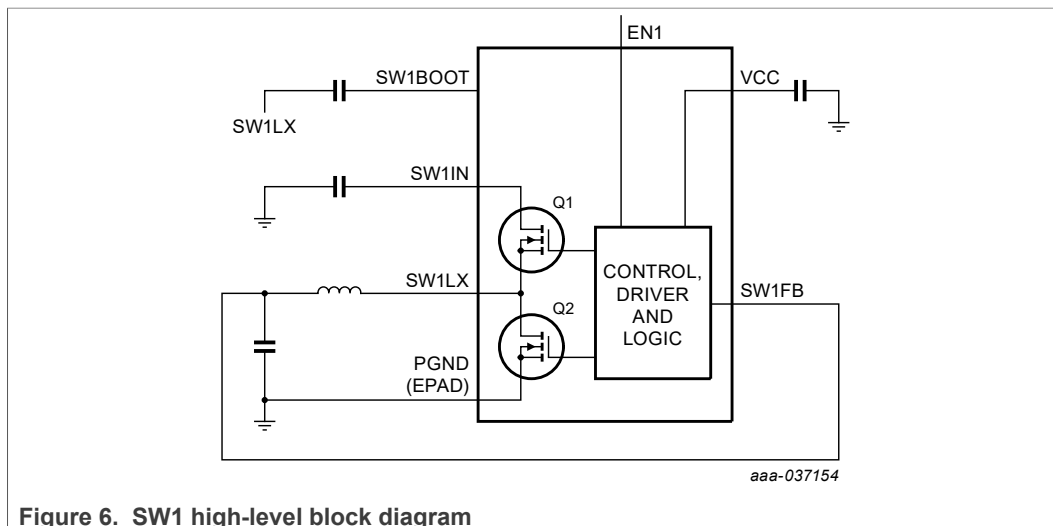
Figure 6. SW1 high-level block diagram
