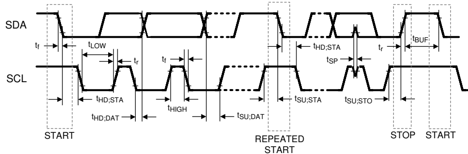
Figure 7-1. I²C Timing
