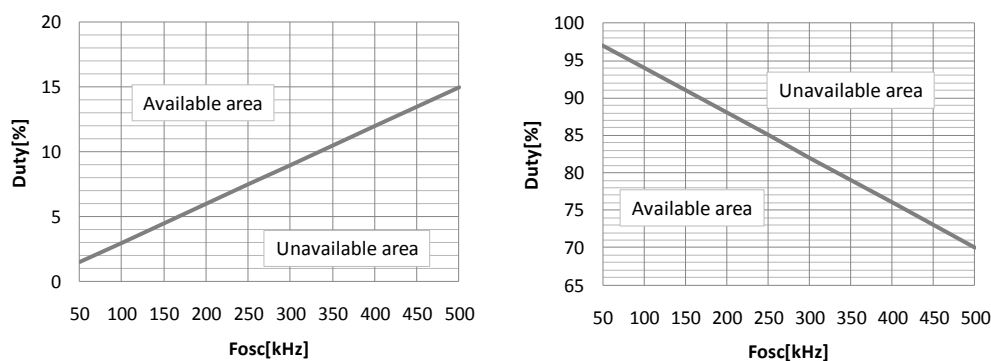
Fig.34 Frequency vs input-output voltage ratio(Duty)
