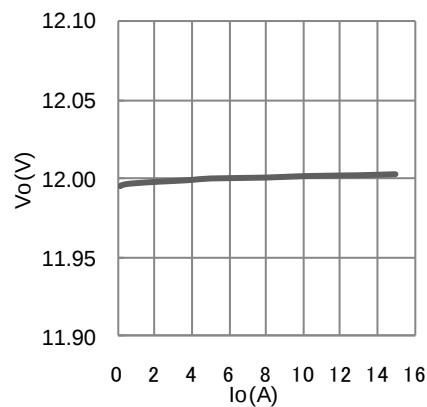
Fig.20 Load Regulation
