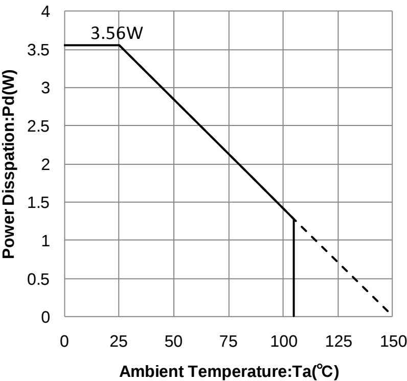
Fig.40 Power Dissipation
