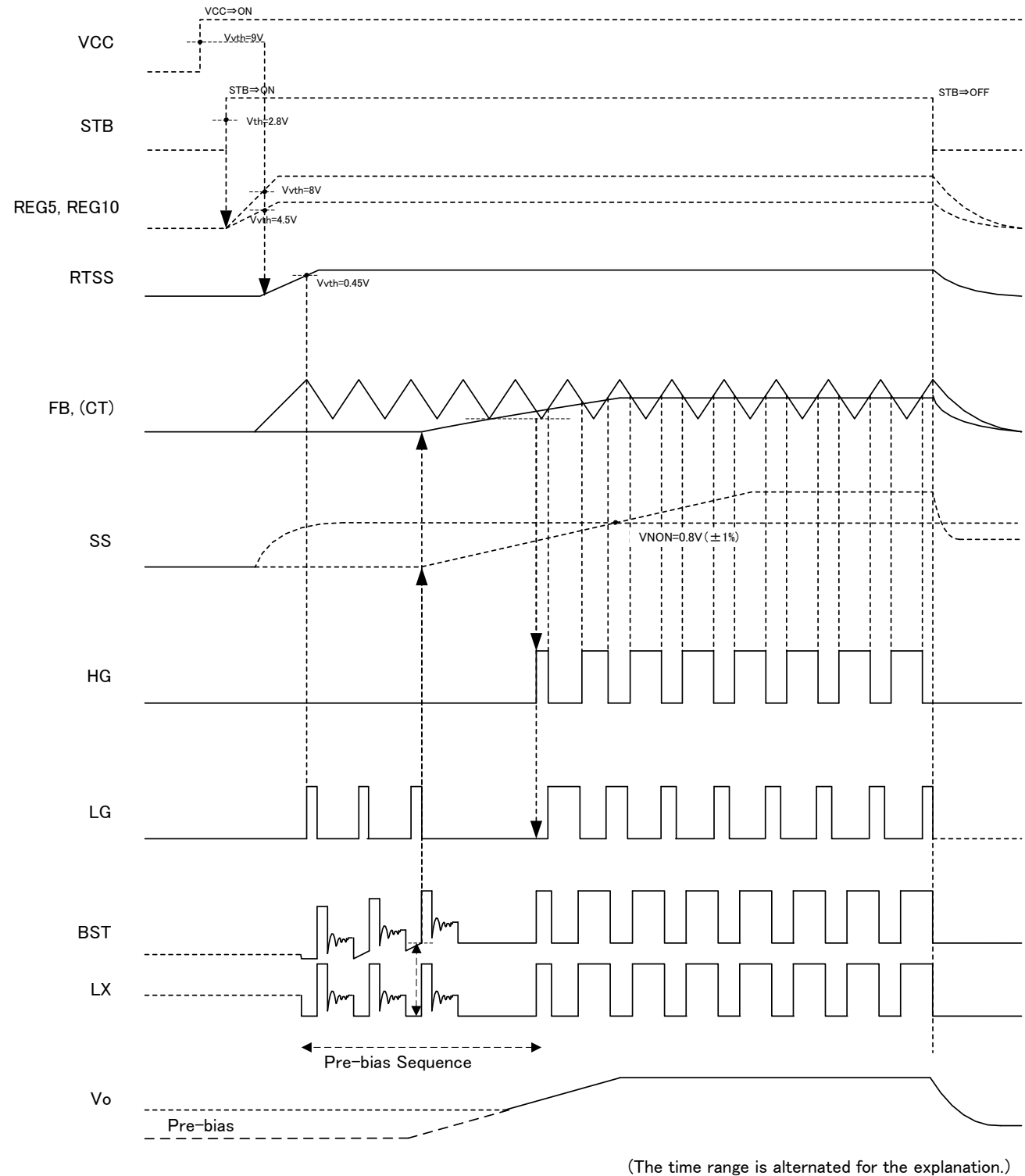
Fig.35 TIMING CHART(START-UP)
