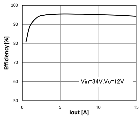
Fig.21 Efficiency
