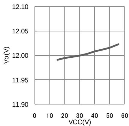
Fig.19 Line Regulation
