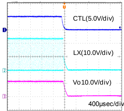
Fig.25 Stop (Rload=2.5Ω)
