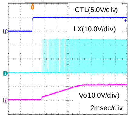
Fig.23 Start-up
