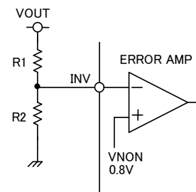
Fig.37 Vout setting
