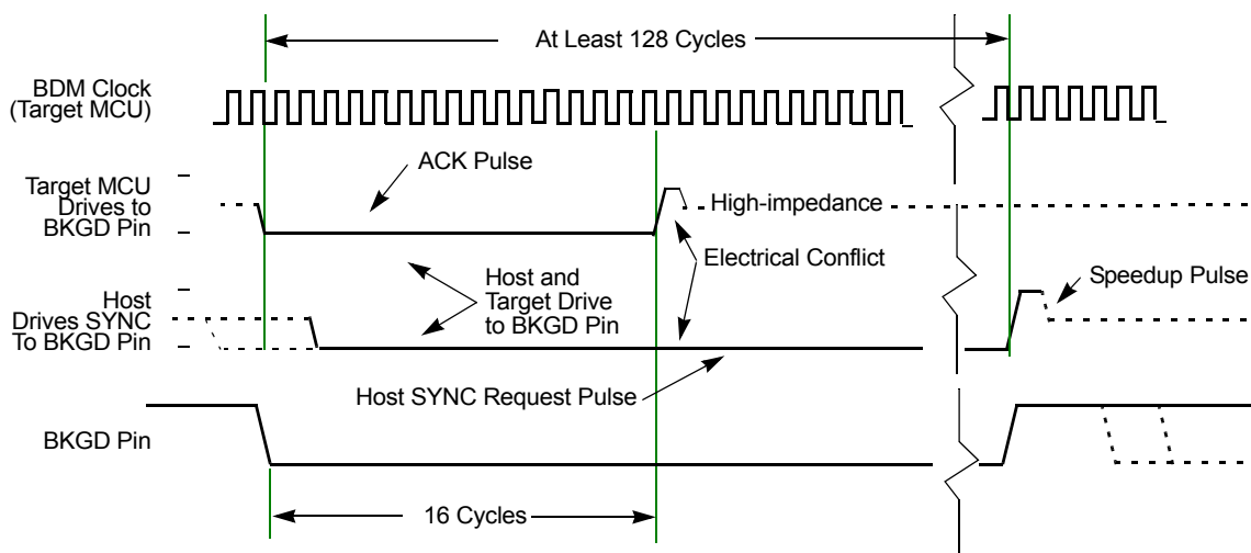
Figure 66. ACK Pulse and SYNC Request Conflict
