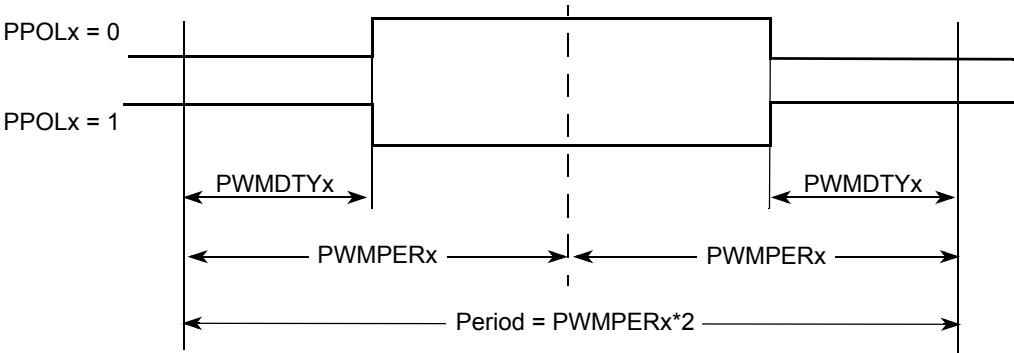
Figure 30. PWM Center Aligned Output Waveform
