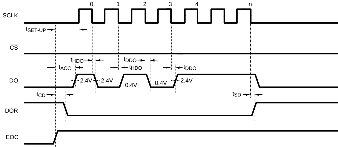
Figure 47. DO Data Output Timing with \overline{\text{CS}} Continuously Low
