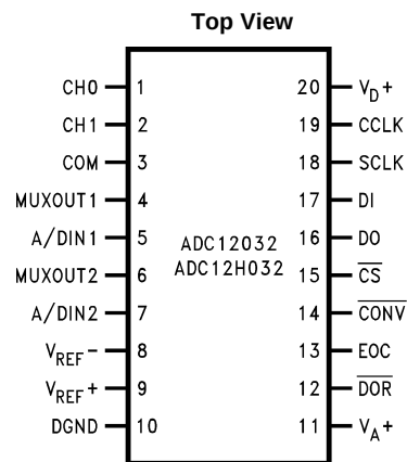
Figure 2. 20-Pin Wide Body SOIC Package See Package Number DW0020B
