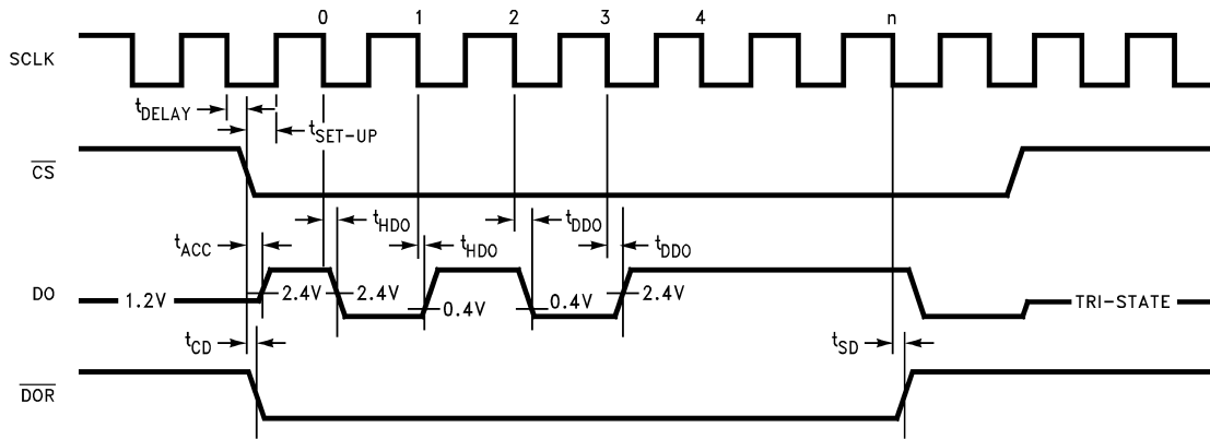
Figure 46. DO Data Output Timing Using \overline{\text{CS}}
