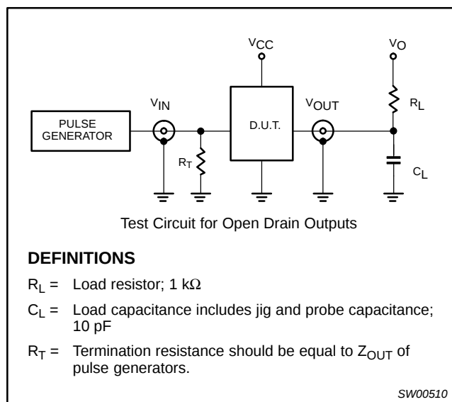
Figure 7. Test circuit
