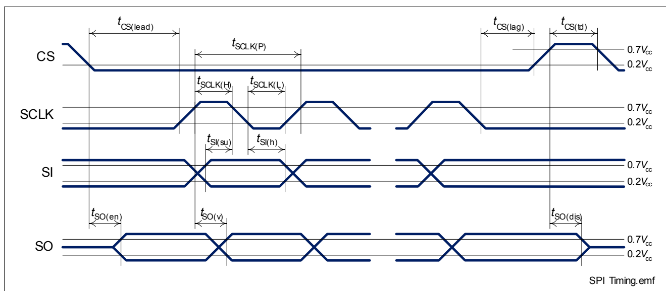
Figure 12 Timing Diagram
