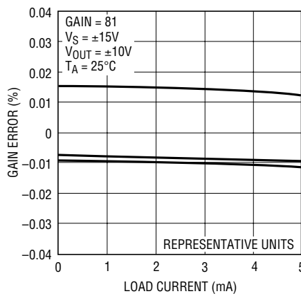
Gain Error vs Load Current
